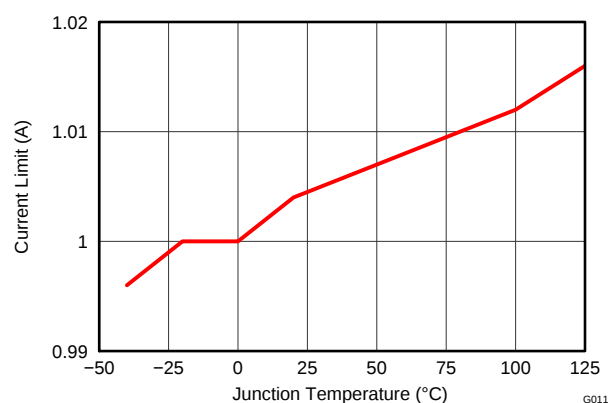
Figure 12. PoE Current Limit vs Temperature
