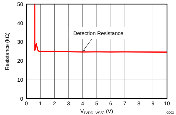
Figure 4. Detection Resistance vs PoE Voltage
