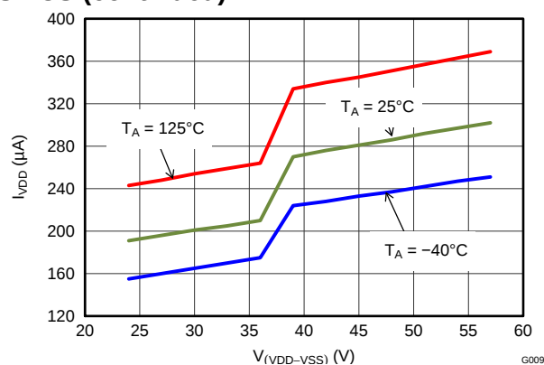
Figure 10. I_VDD Bias Current vs Voltage
