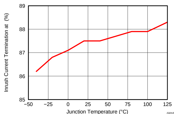
Figure 14. Inrush Termination Threshold vs Temperature
