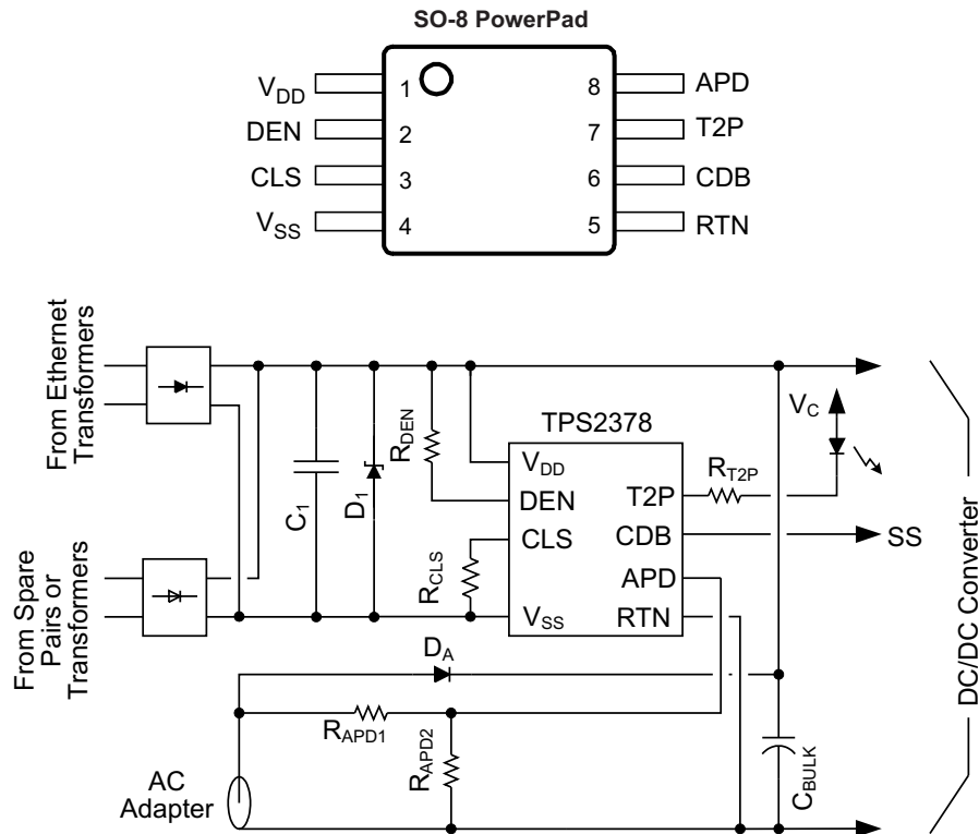
Figure 1. Typical Application
